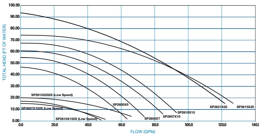
SUPER PUMP FLOW VS. TOTAL HEAD
